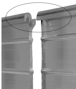
Telescopic-connection without screws
